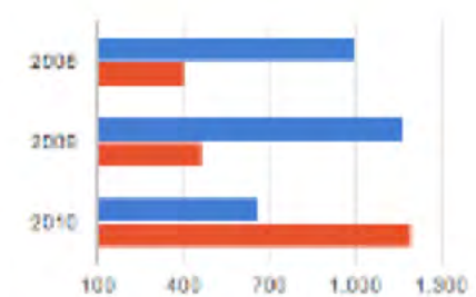
Bar Chart
