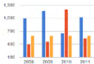
Column Chart
