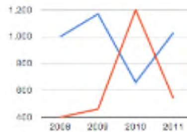
Line Chart
