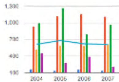
Combo Chart
