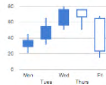
Candlestick Chart
